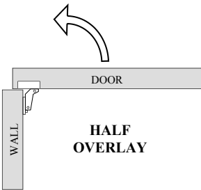
HINGE DOOR SETUP HOLE DEPTH VARIES BETWEEN CONCEALED HINGE TYPES
