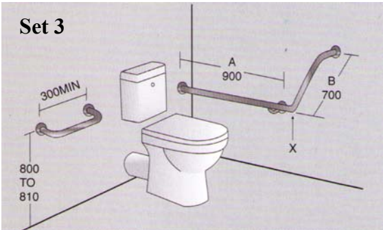
Set 3 SIDE & REAR WALL FIX 30 Deg RAIL BEND X TO BE 100 - 150mm FORWARD OF PAN RIM
