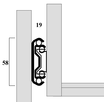
DRAWER CROSS SECTION
