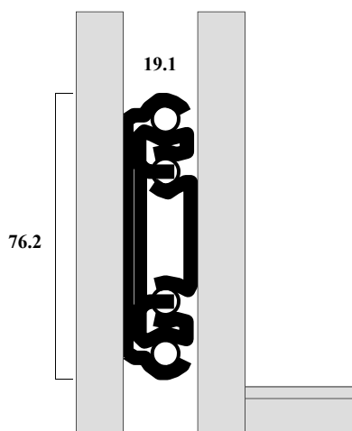
DRAWER CROSS SECTION
