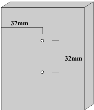
MOUNTING PLATE SETUP FOR OVERLAY & HALF OVERLAY DOORS. ADD DOOR THICKNESS FOR INSET DOORS.
