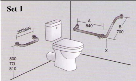
Set 1 SIDE WALL 30 Deg RAIL BEND X TO BE 100 - 150mm FORWARD OF PAN RIM
