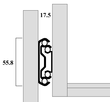
DRAWER CROSS SECTION
