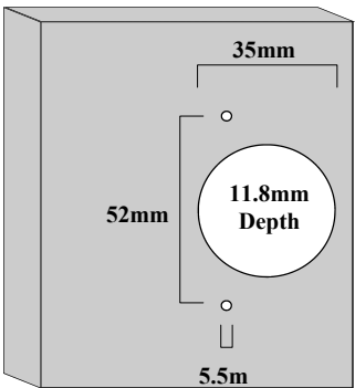
HINGE DOOR SETUP HOLE DEPTH VARIES BETWEEN CONCEALED HINGE TYPES
