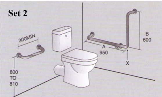
Set 2 SIDE WALL 90 Deg RAIL BEND X TO BE 200 - 250mm FORWARD OF PAN RIM
