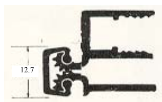
Shower Screen Hinge for hinging Glass to aluminium frame. To suit 6mm glass with neo rubber.
