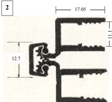
Shower Screen Hinge for hinging 6mm glass to 6mm glass with neo rubber.
