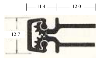
Cabinet or Shower Screen Hinge For panels or extrusions 12mm thick.
