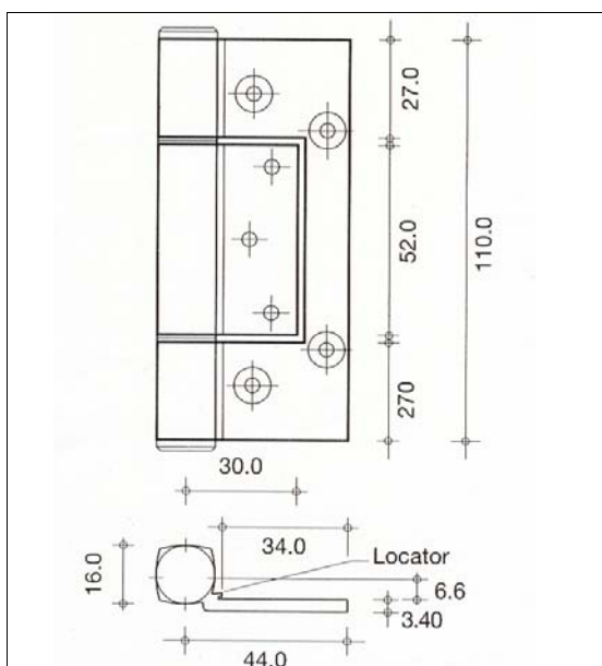
FIXED PIN FLAT
